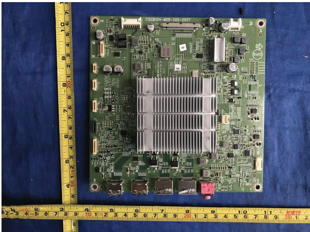
Figure 12. Main board 715GB104
