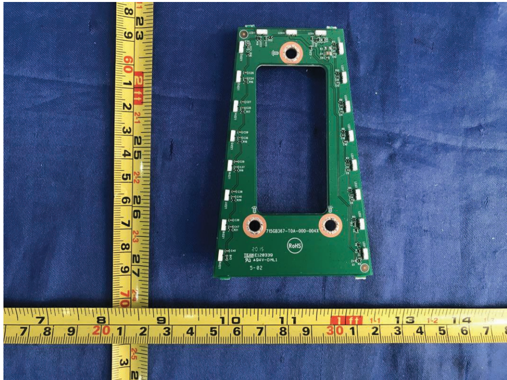
Figure 17. LED driver board 715GB367
