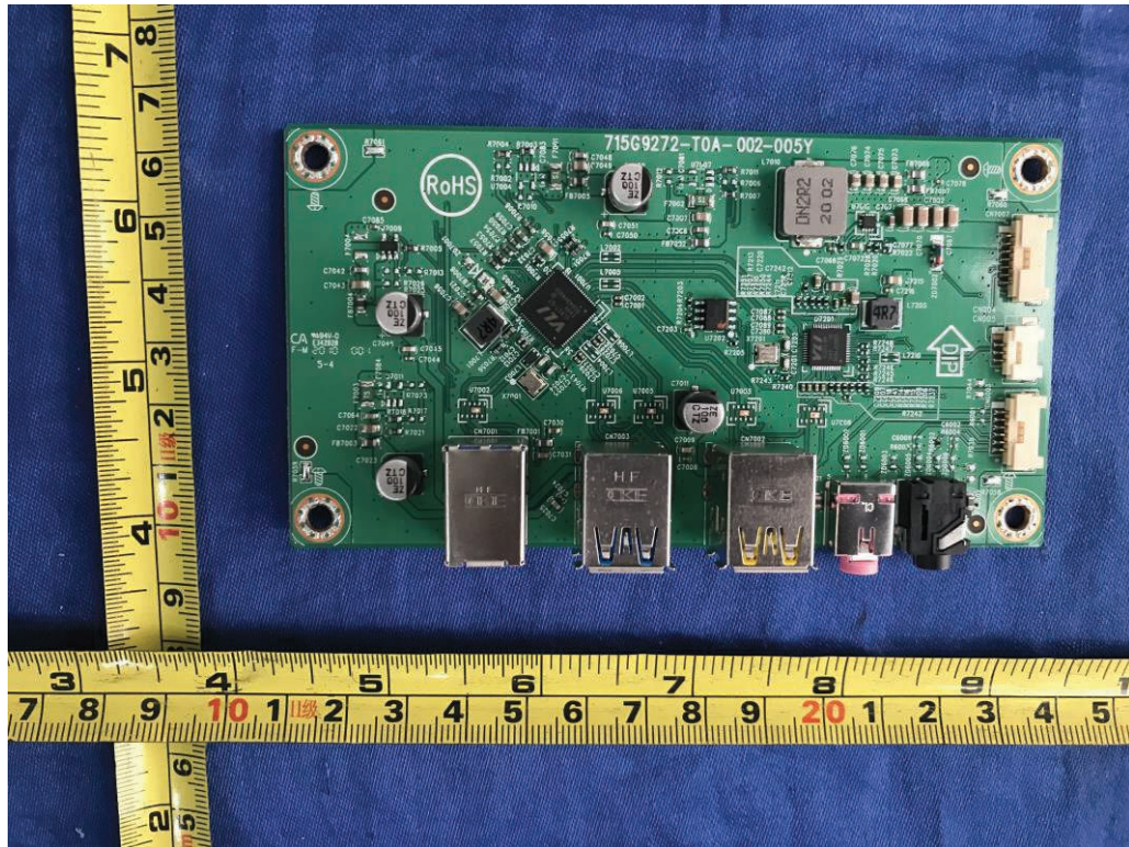
Figure 15. USB board 715G9272
