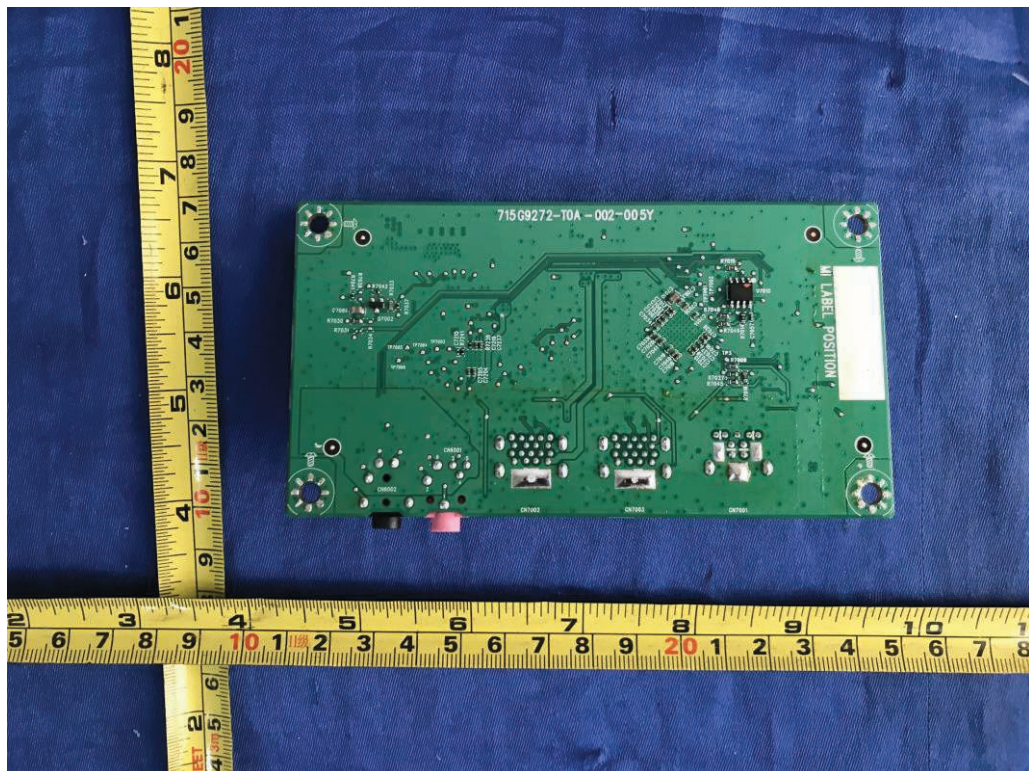
Figure 14. USB board 715G9272
