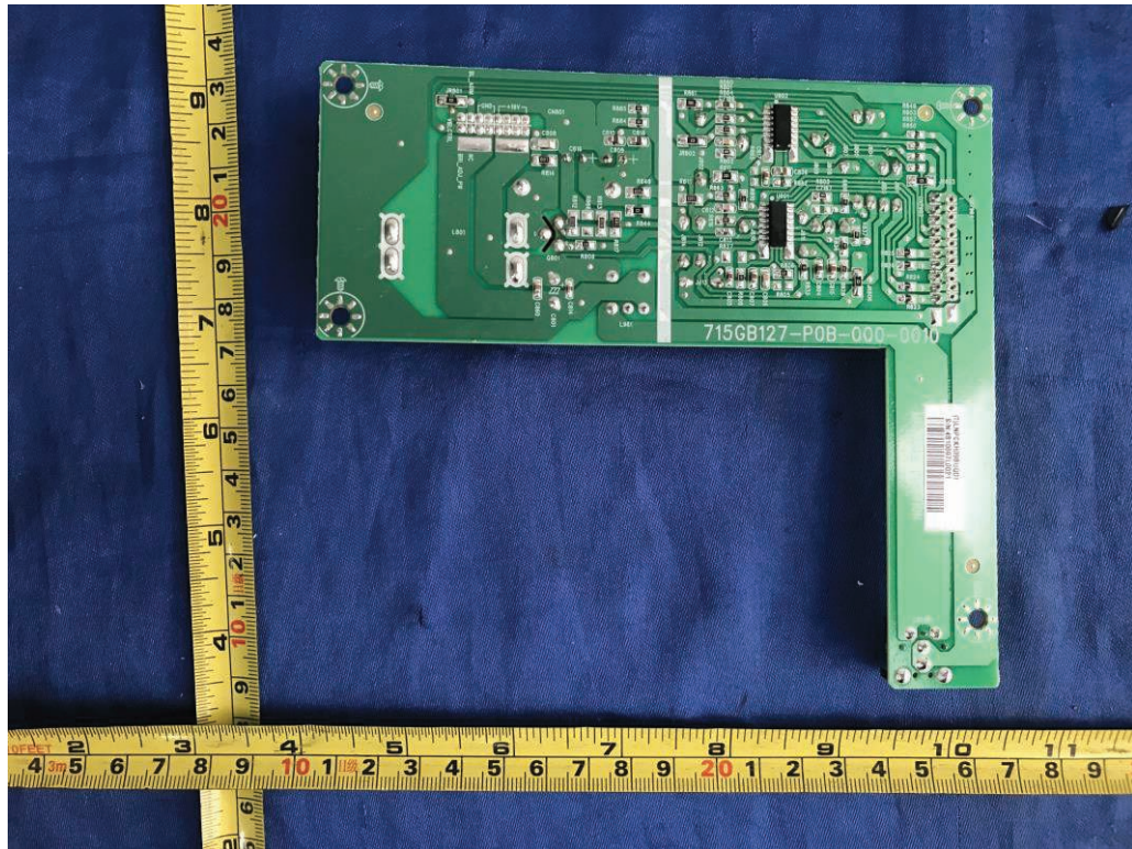
Figure 9. DC converter board 715ZGB127
