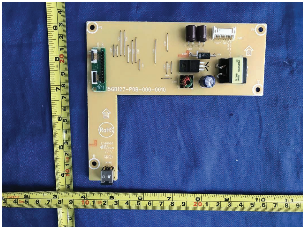
Figure 10. DC converter board 715ZGB127
