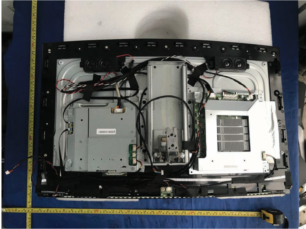
Figure 3. Internal view
