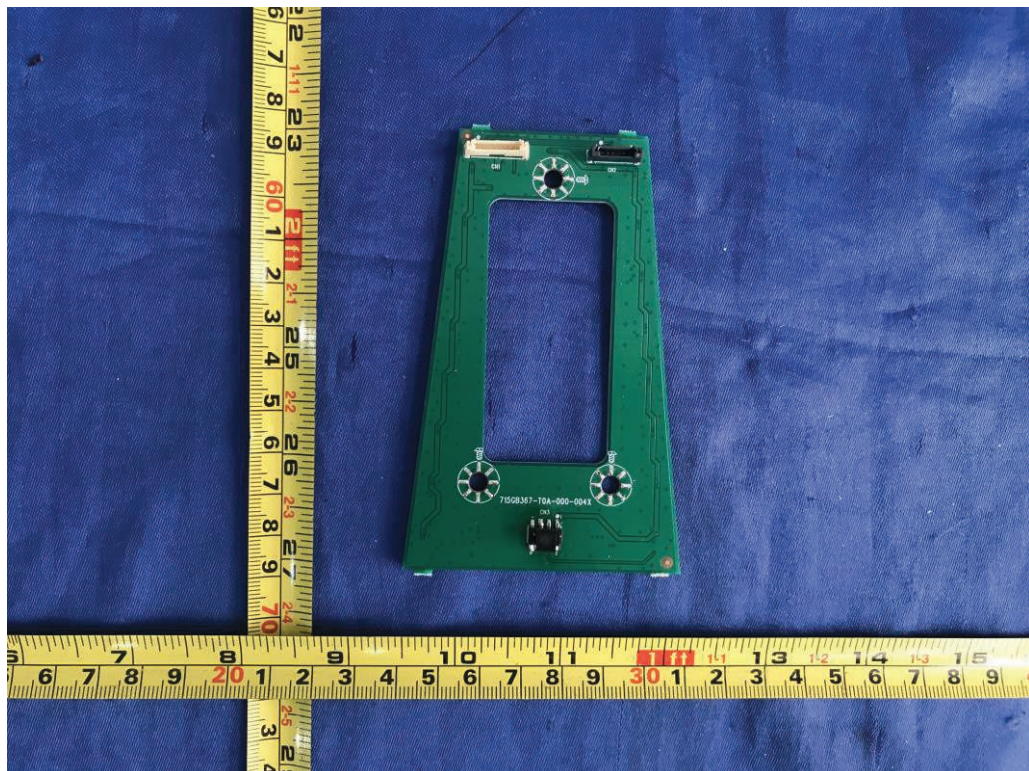
Figure 18. LED driver board 715GB367
