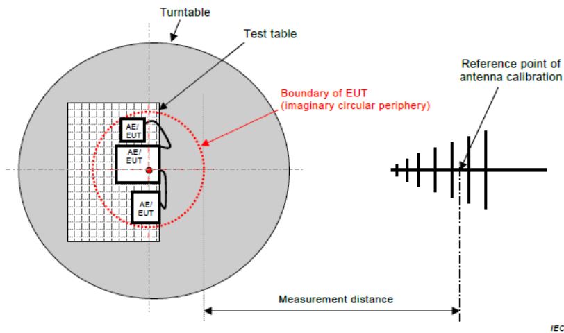
Figure C.1 – Measurement distance
