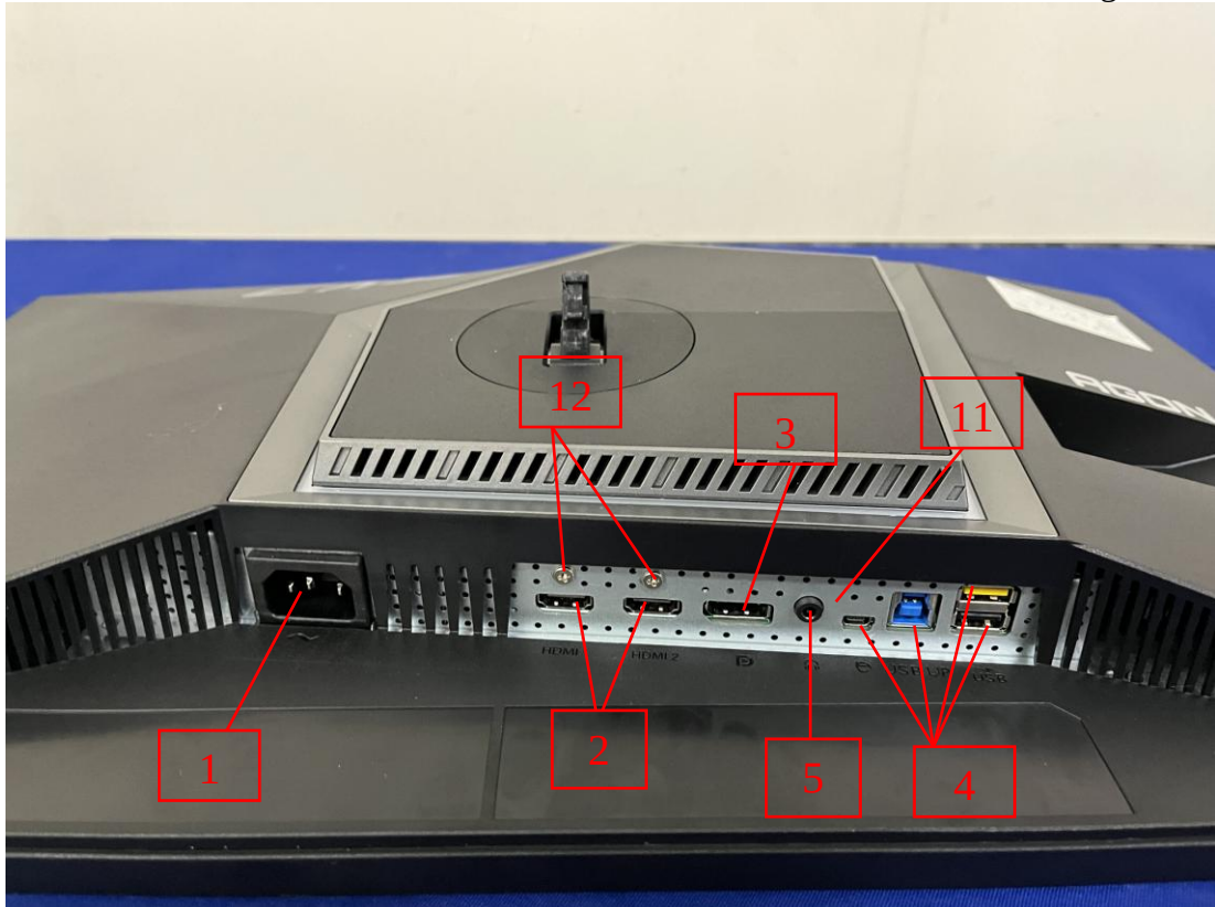
ESD Figure 3 Signal Port of the EUT
