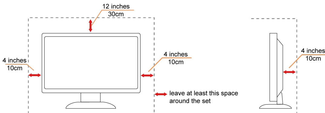
Installd with stand
